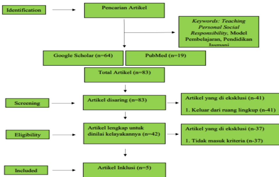
Gambar 1. PRISMA Flowchart
